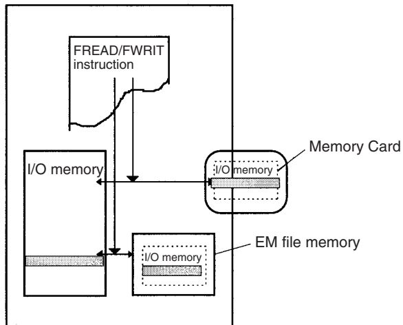
FREAD(700)/FWRIT(701): Transfers between I/O memory and file memory CPU Unit
