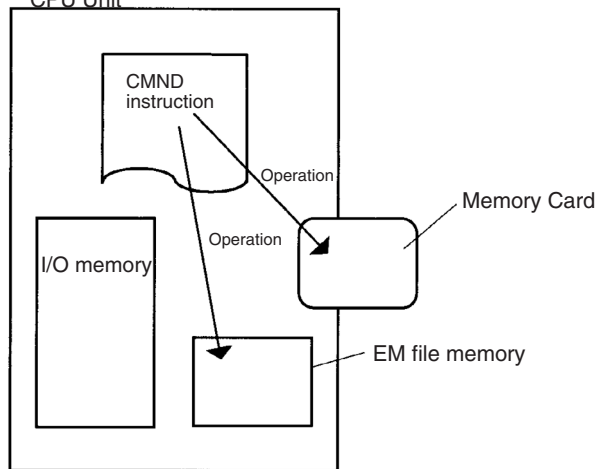
CMND(490): File memory operations (Not possible for CS-series CPU Units that are pre-EV1) CPU Unit
